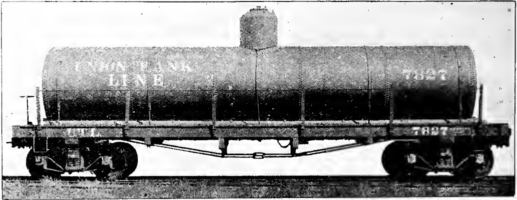
Fig. 48. TANK CAR FOR OIL, ACIDS, MOLASSES, ETC. UNION TANK LINES. Length, 37 ft. Capacity, 8,000 gals. Weight, 28,000 lbs. (Details are shown in Figs. 373-375.)
